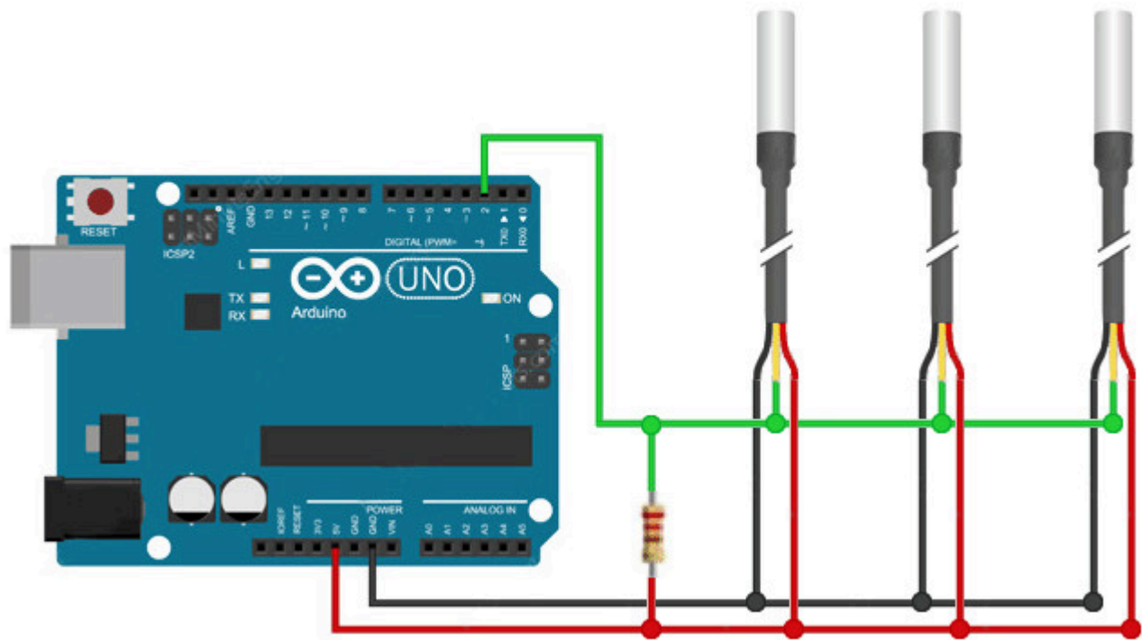
Conexão 1 Wire Sensor DS18B20 Inox
